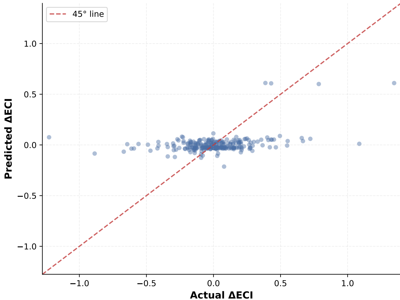
Random Forest — \Delta ECI | Test R^2=0.154 RMSE=0.2364
