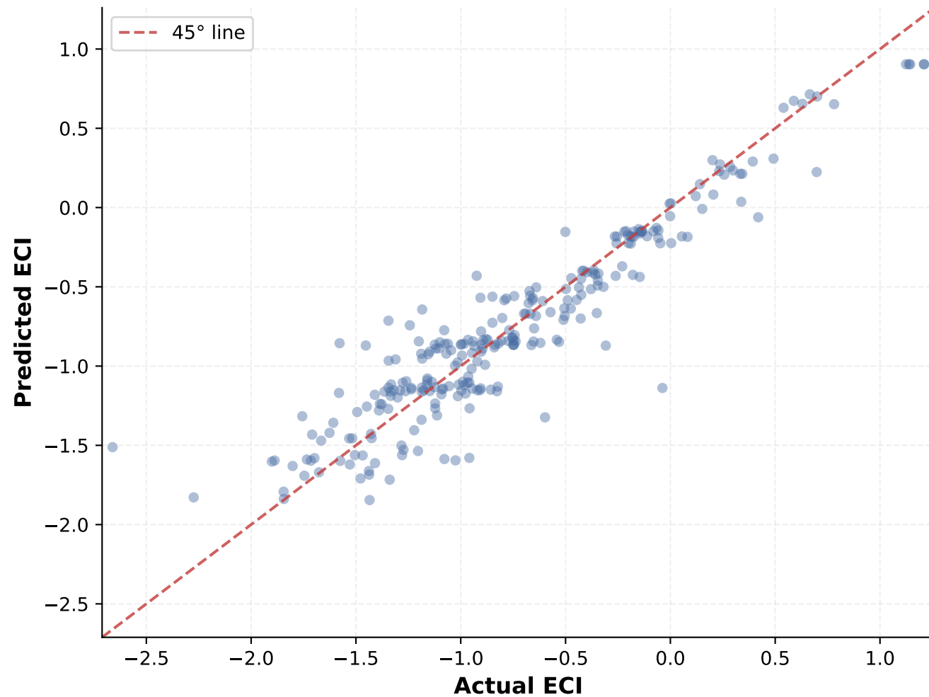
Random Forest — ECI | Test R^2=0.876 RMSE=0.2290
